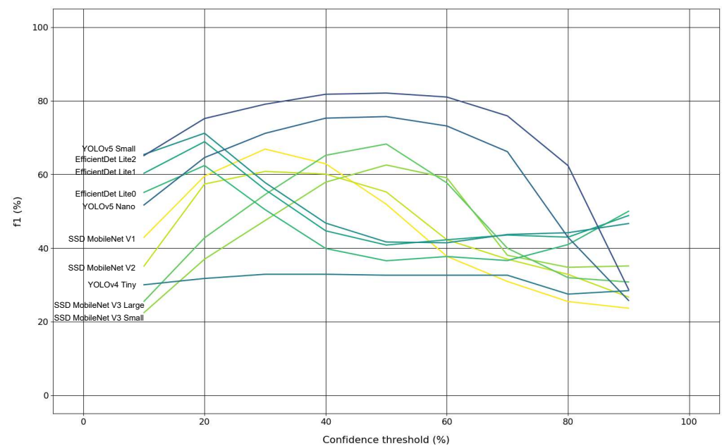
Figure 7. Evolution of F1 score of the quantised models, with maximum input resolutions, over several confidence thresholds.
