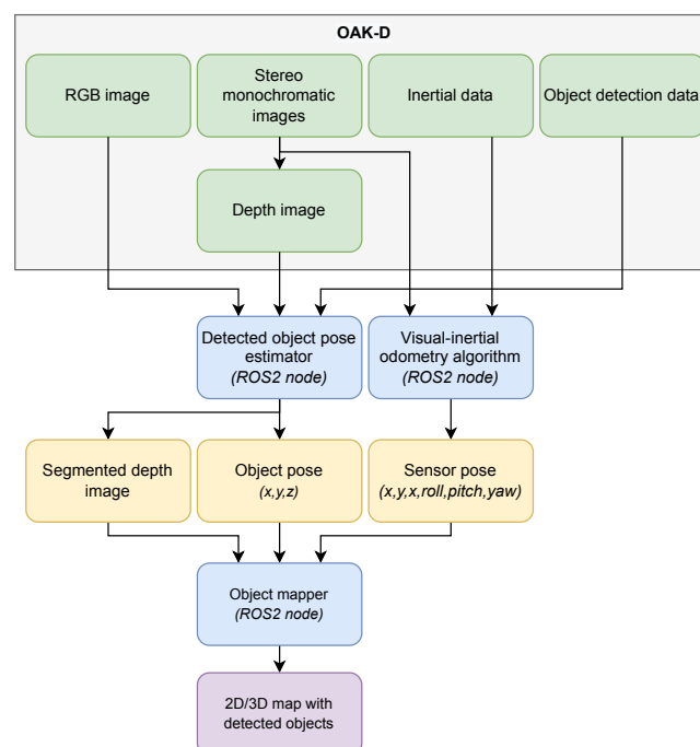
Figure 2. Tree trunk mapping algorithm diagram: green blocks are data provided by sensors, yellow blocks are computational data, blue blocks are computational nodes, and purple blocks are results. The computational nodes have been developed in ROS2, of which, one of them computes the detected object XYZ pose, the other corresponds to a visual-inertial odometry algorithm that estimates the sensor's six DoF poses, and the last one uses the information given by the latter two and maps the detected objects.
