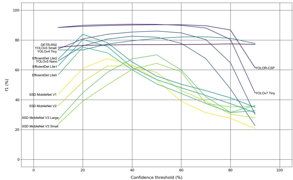
Figure 5. Evolution of F1 score of the non-quantised models, with their default input resolutions, over several confidence thresholds.
