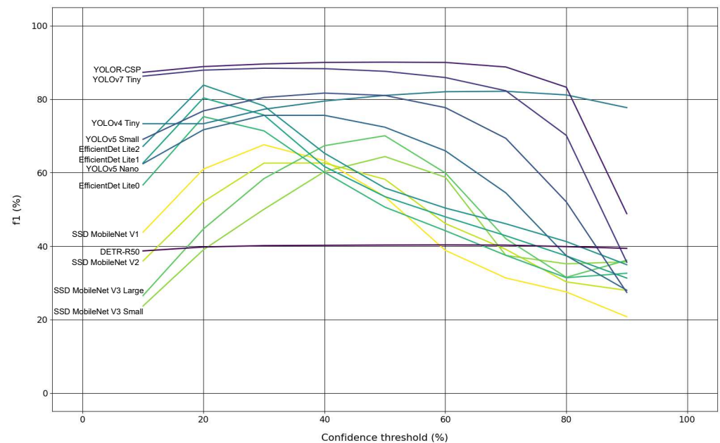
Figure 6. Evolution of F1 score of the non-quantised models, with minor input resolutions, over several confidence thresholds.
