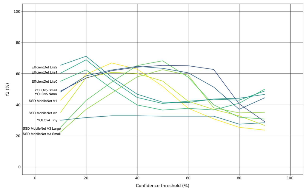
Figure 8. Evolution of F1 score of the quantised models, with minor input resolutions, over several confidence thresholds.
